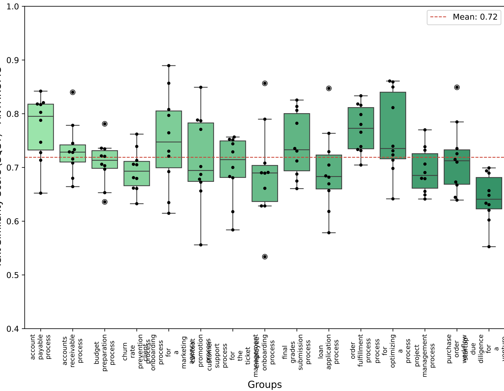
Text Similarity Score (SQST) - ANTHROPIC
